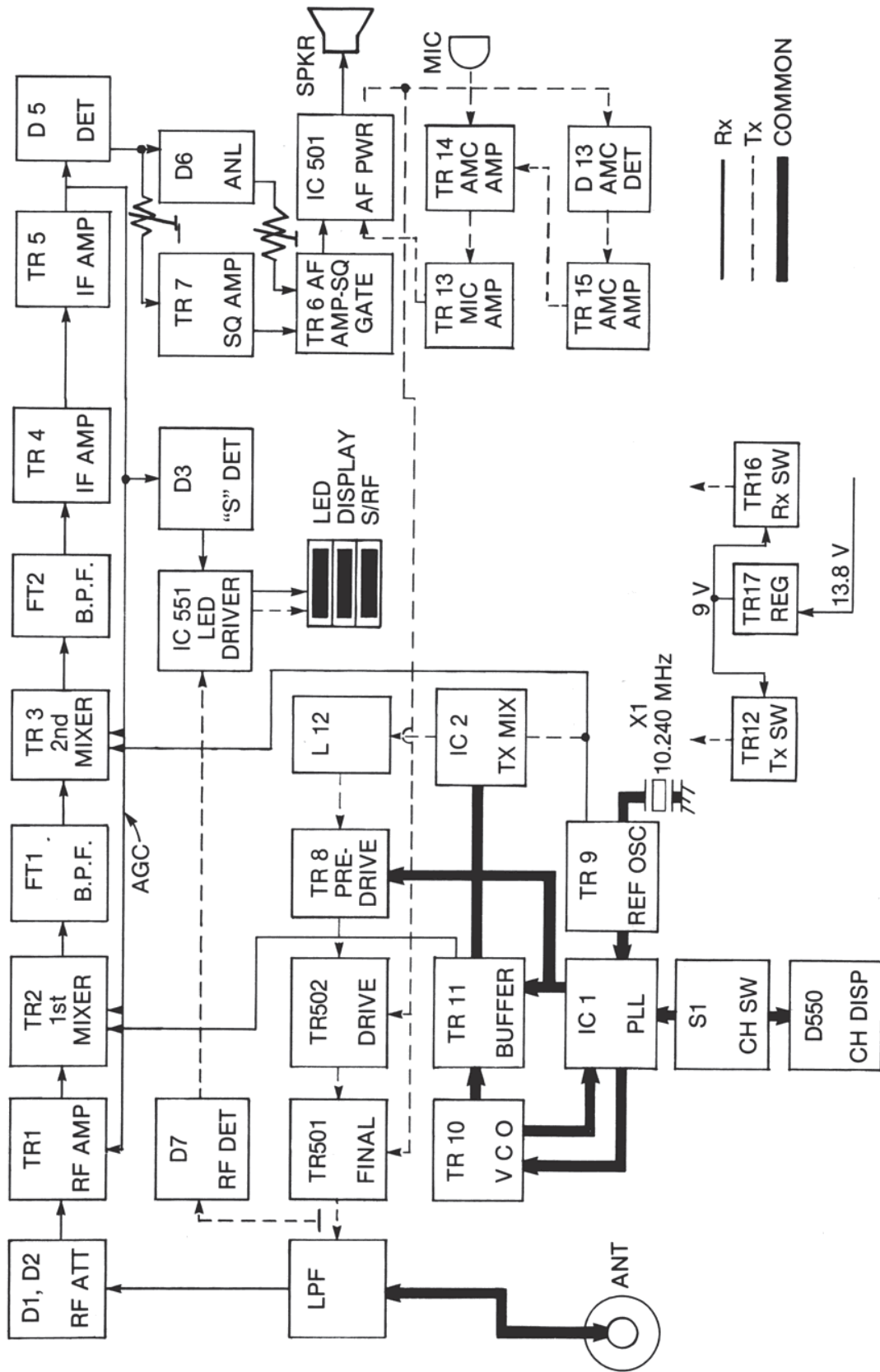
PC 33 BLOCK DIAGRAM
