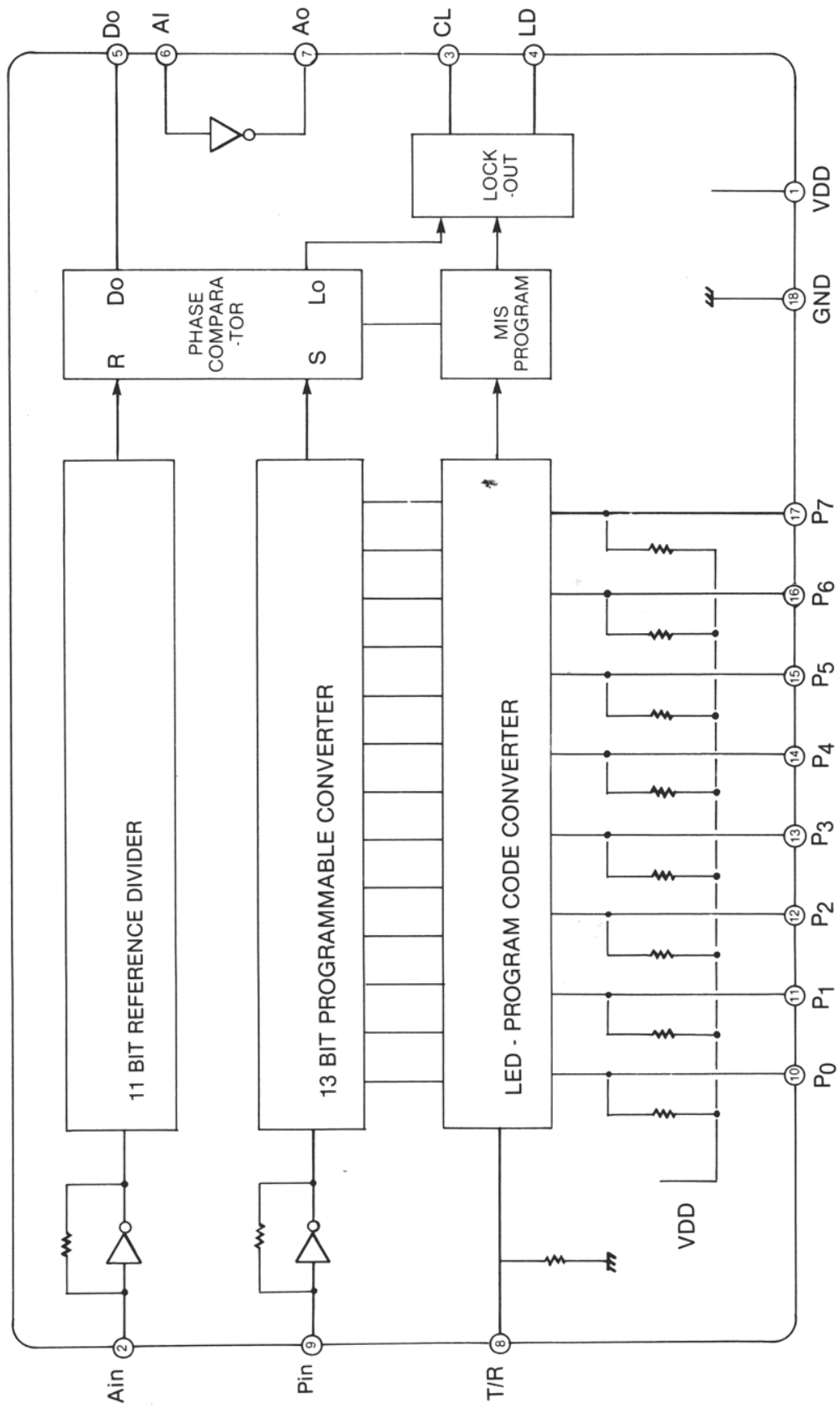
PLL BLOCK DIAGRAM (IC 1)
